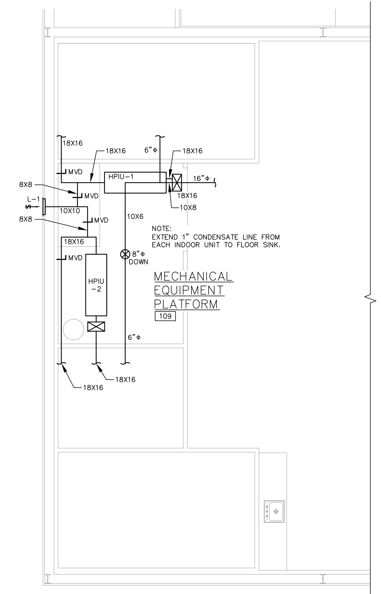
MECHANICAL PLATFORM PLAN SCALE: 1/4"=1'-0"
