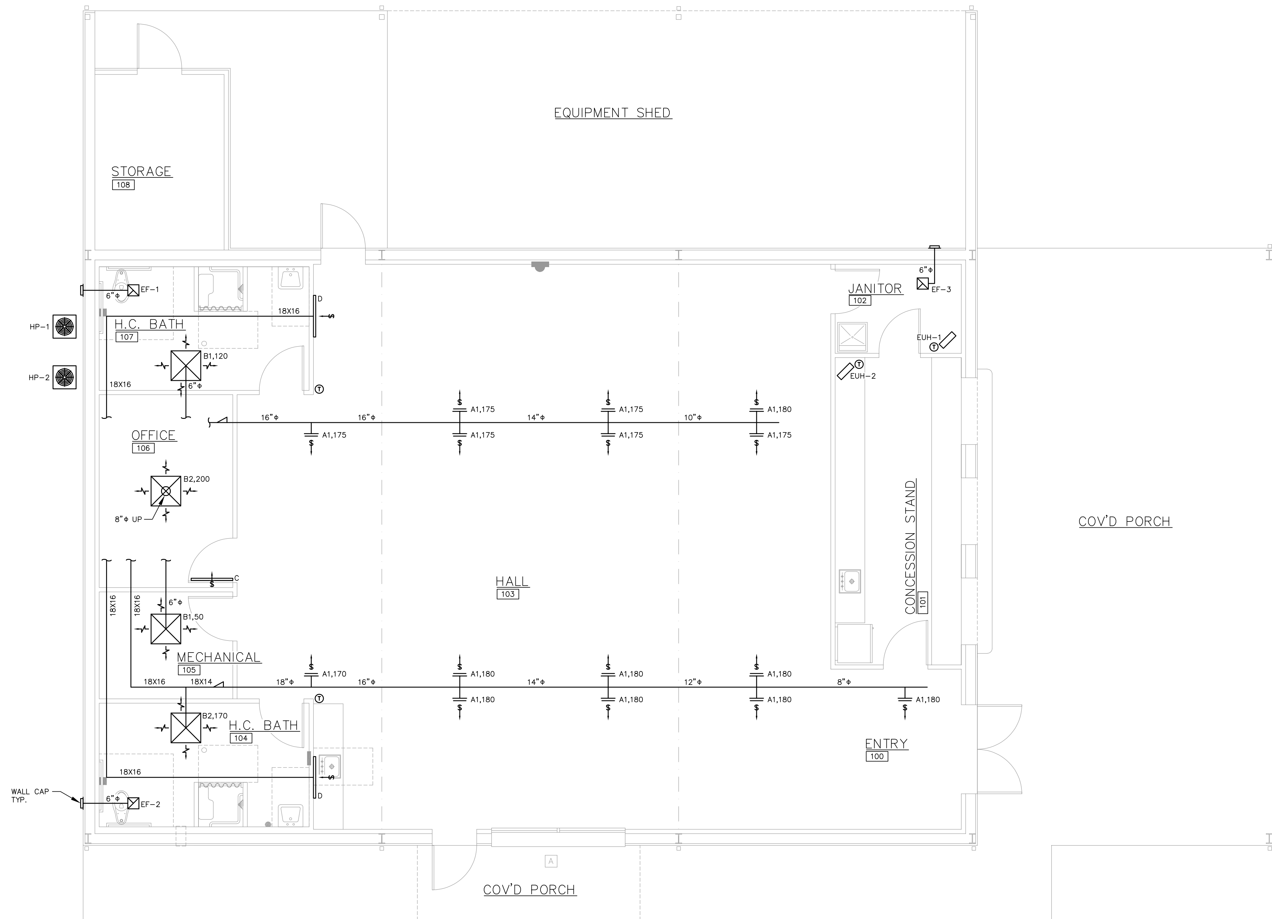
FLOOR PLAN - HVAC SCALE: 1/4"=1'-0"
