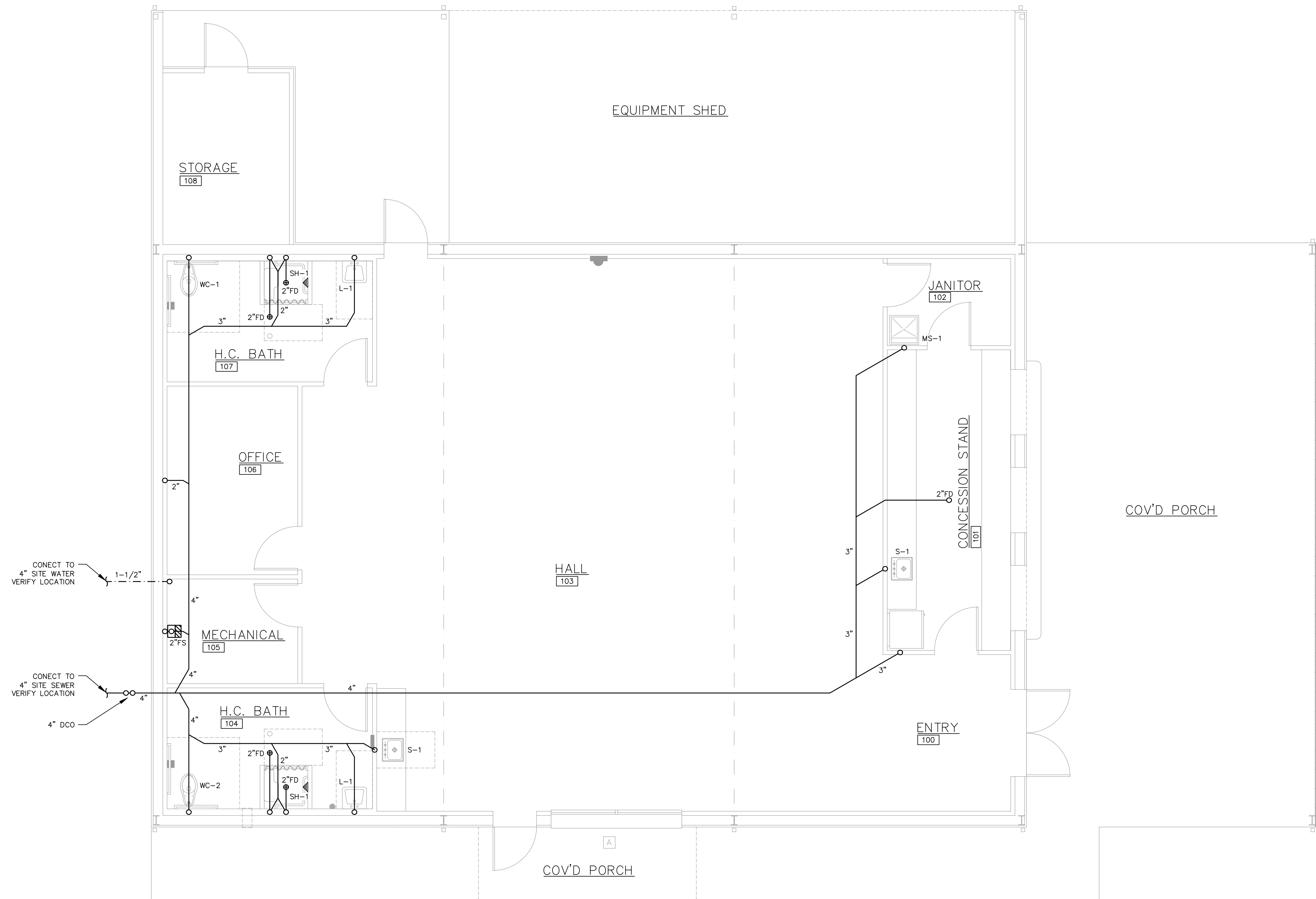
FLOOR PLAN — PLUMBING UNDER FLOOR SCALE: 1/4"=1'-0"
